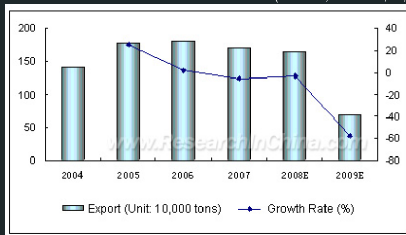
Statistics and Forecast of China Sodium Carbonate Export, 2004-2009 (Unit: 10, 000 tons, %.)
